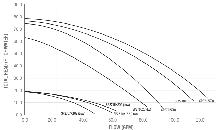
MAX-FLO II FLOW VS TOTAL HEAD
